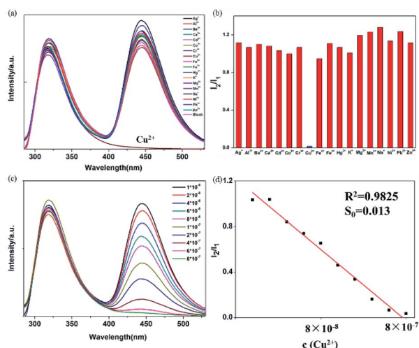
Fig. 6 (a) Fluorescence spectra of BBM-PMO-10 ( 5 \times 10^{-6} g mL ^{-1} ) with different metal ions ( 10^{-6} M) in THF/H _2 O = 3 : 7 (v/v); (b) fluorescence intensity ratio I_2/I_1 of BBM-PMO-10 ( 5 \times 10^{-6} g mL ^{-1} ) with different metal ions ( 10^{-6} M) in THF/H _2 O = 3 : 7 (v/v); (c) fluorescence spectra of BBM-PMO-10 in THF/H _2 O = 3 : 7 (v/v) with different concentrations of Cu ^{2+} ( 10^{-8} – 8 \times 10^{-7} M); (d) linear relationship between I_2/I_1 of BBM-PMO-10 ( 5 \times 10^{-6} g mL ^{-1} ) and the concentration of Cu ^{2+} in the solvent.
