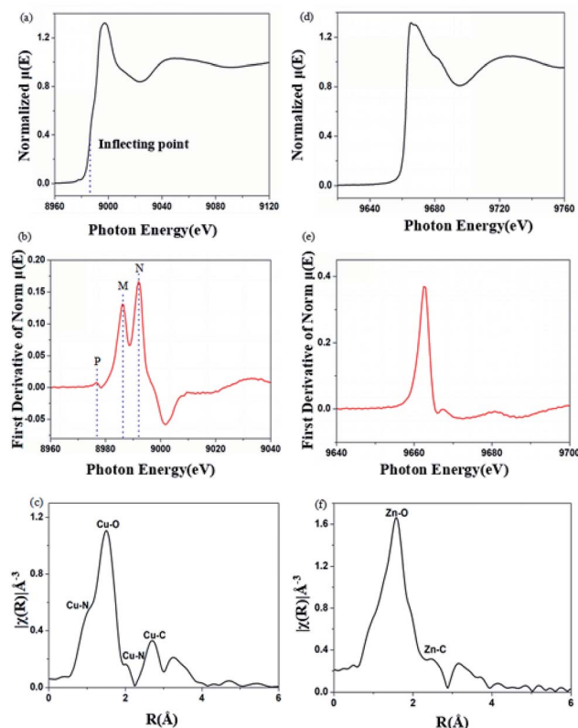
Fig. 7 (a) Normalized XANES spectrum at the copper K-edge; (b) corresponding first derivate XANES spectrum; (c) Fourier transformed extended X-ray absorption fine structure spectrum (EXAFS) of Cu 2+ -chelated BBM-PMO-10. (d) Normalized XANES spectrum at the Zn K-edge; (e) corresponding first derivate XANES spectrum; (f) Fourier transformed extended X-ray absorption fine structure spectrum (EXAFS) of Zn 2+ -chelated BBM-PMO-10.
