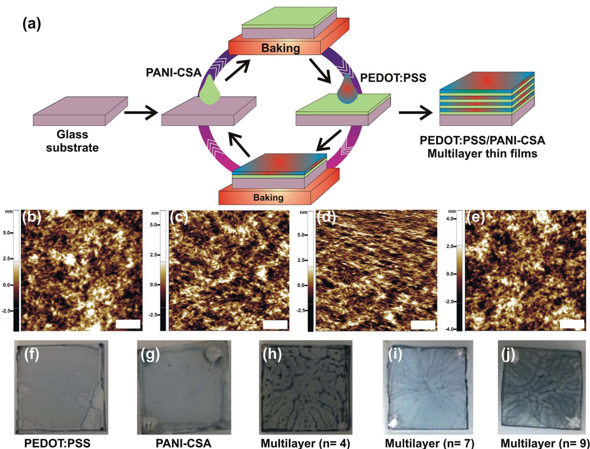
Fig. 1 (a) The schematic showing the deposition of PEDOT:PSS/PANI-CSA ML thin films via layer-by-layer deposition technique. After the deposition of the ML thin films the top layer PEDOT:PSS is treated with DMSO to further enhance the conductivity. (b–e) AFM images of the ML thin films deposited at a spin speed of 4000, 5000, 7000, and 9000 rpm, respectively. The scale bar is 200 nm. (f–j) Digital photographs of the PEDOT:PSS, PANI-CSA, and PEDOT:PSS/PANI-CSA ML thin films deposited at a spin speed of 7000 rpm.
