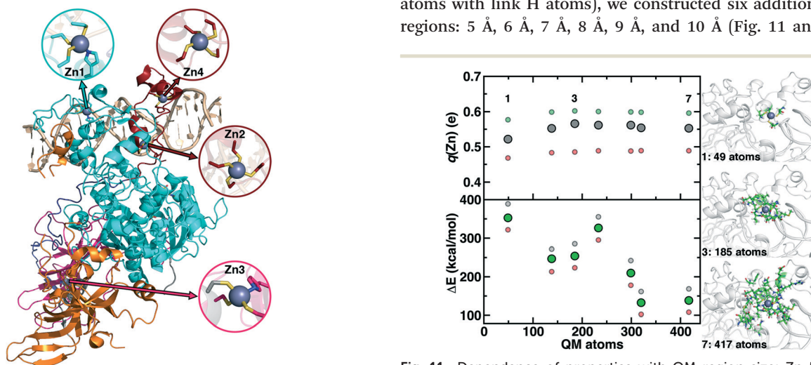
Fig. 10 Structure of DNMT1 with DNA bound and separately colored protein chains. Each of the Zn sites in the crystal structure is shown in an inset with the relevant site on the protein indicated by arrows. Zn site numbering corresponds to the numbering in the experimental crystal structure. Zn is shown as a gray sphere, Cys S is shown in yellow, His N is shown in blue, and carbon atoms are colored according to the chain to which they belong.
