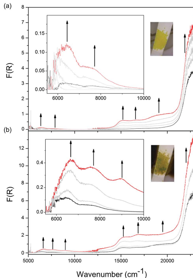
Fig. 4 Solid state Vis-NIR SEC of 1-Zn in 0.1 M [n\text{-Bu}_4\text{N}]\text{PF}_6/\text{MeCN} with arrows indicating progression of spectral bands at an applied potential of (a) -2.1\text{ V} ; (b) -2.4\text{ V} , with insets showing the NIR region as well as photos displaying the colour of the frameworks at respective potentials.
