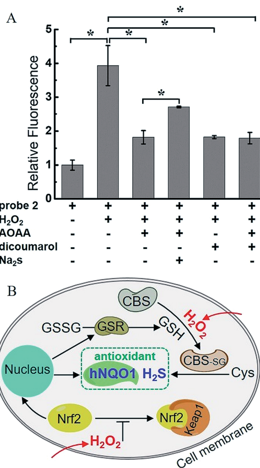
Fig. 8 (A) Relative fluorescence intensity of confocal microscopy images from H 2 O 2 -induced HeLa cells. N = 3 fields of cells, error bars are means ± sd. * P < 0.05. (B) A proposed mechanism of the synergistic antioxidant effect of H 2 S and hNQO1 under oxidative stress.
