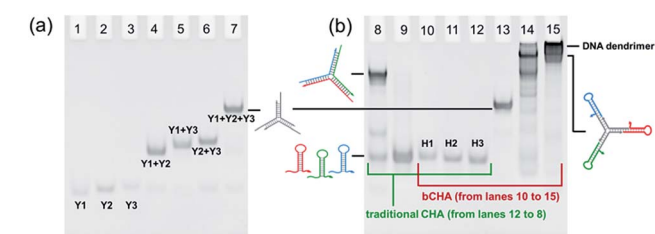
Fig. 2 Native PAGE to demonstrate (a) the formation of Y-scaffold DNA and (b) the reaction mechanism of traditional CHA for assembly of three-arm DNA junctions (lanes 8–12) and bCHA for assembly of DNA dendrimers (lanes 10–15). Lanes 8–12: H1 + H2 + H3 + initiator to form a three-arm DNA junction, H1 + H2 + H3, H1, H2 and H3, respectively; lane 13: Y-scaffold DNA; lane 14: Y-scaffold DNA + H1 + H2 + H3 to form hairpin trimer; lane 15: hairpin trimer + initiator to form a DNA dendrimer. The initial concentration of each DNA species is 10 \mu\text{M} . The experiments are implemented in TE buffer (10 mM Tris-HCl, 1 mM EDTA-2Na and 12.5 mM \text{MgCl}_2 , pH 8.0) with a final volume of 12 \mu\text{L} .
