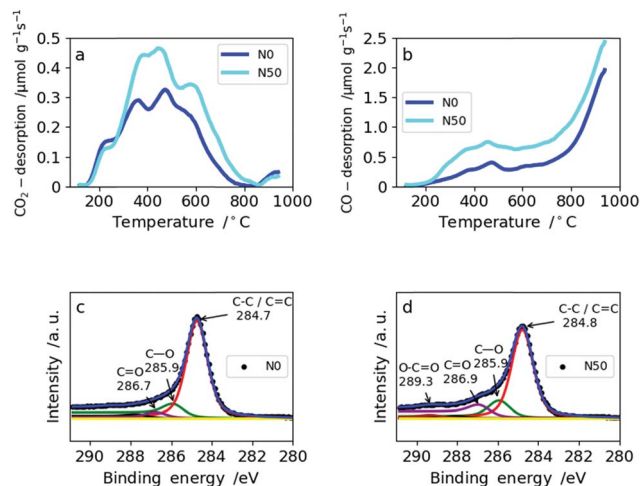
Fig. 4 TPD spectra for N0 and N50: (a) \text{CO}_2 desorption rates from TPD, (b) \text{CO} desorption from TPD, XPS spectra for N0 and N50: (c) N0 and (d) N50.
