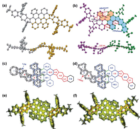
Fig. 3 Top view and side view of the X-ray crystallographic structure of (a) compound 9 (precursor for PH 1 ) and (b) tetradicaloid 2 ; the hydrogen atoms are omitted for clarity. Selected bond lengths (Å) and calculated NICS(1) av values in the rings A–I of (c) 1 and (d) 2 . Calculated ACID plots of (e) 1 and (f) 2 . Isovalue is 0.05, and the blue and red arrows indicate diamagnetic and paramagnetic ring current flows, respectively.
