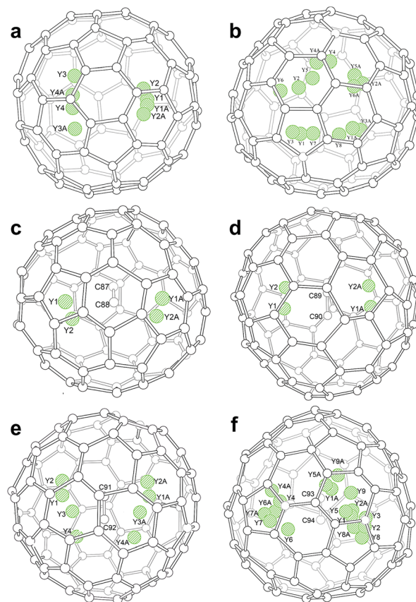
Fig. 1 Perspective drawings showing the internal yttrium sites. (a) 8 in \text{Y}_2@C_{s(6)}-C_{82} , (b) 14 in \text{Y}_2@C_{3v(8)}-C_{82} , (c) 4 in \text{Y}_2C_2@C_{s(15)}-C_{86} , (d) 4 in \text{Y}_2C_2@C_{1(26)}-C_{88} , (e) 8 in \text{Y}_2C_2@C_{2(41)}-C_{90} , and (f) 17 in \text{Y}_2C_2@C_{2(61)}-C_{92} .
