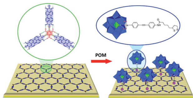
Fig. 13 Schematic depiction of the organisational preferences of the Keggin-type POM-based inorganic-organic hybrid units [\text{PW}_{11}\text{O}_{39}\text{Ge}\{p\text{-C}_6\text{H}_4\text{-C}\equiv\text{C-C}_6\text{H}_4\text{-NHC(O)(CH}_2)_4\text{-CH-(CH}_2)_2\text{S-S-}}\}]^{4-} (right) on the PTCDI/melamine-templated gold surface (left). Colour code: W, blue; P, green polyhedra; O, red spheres. Adapted with permission from ref. 29. Copyright 2016 American Chemical Society.
