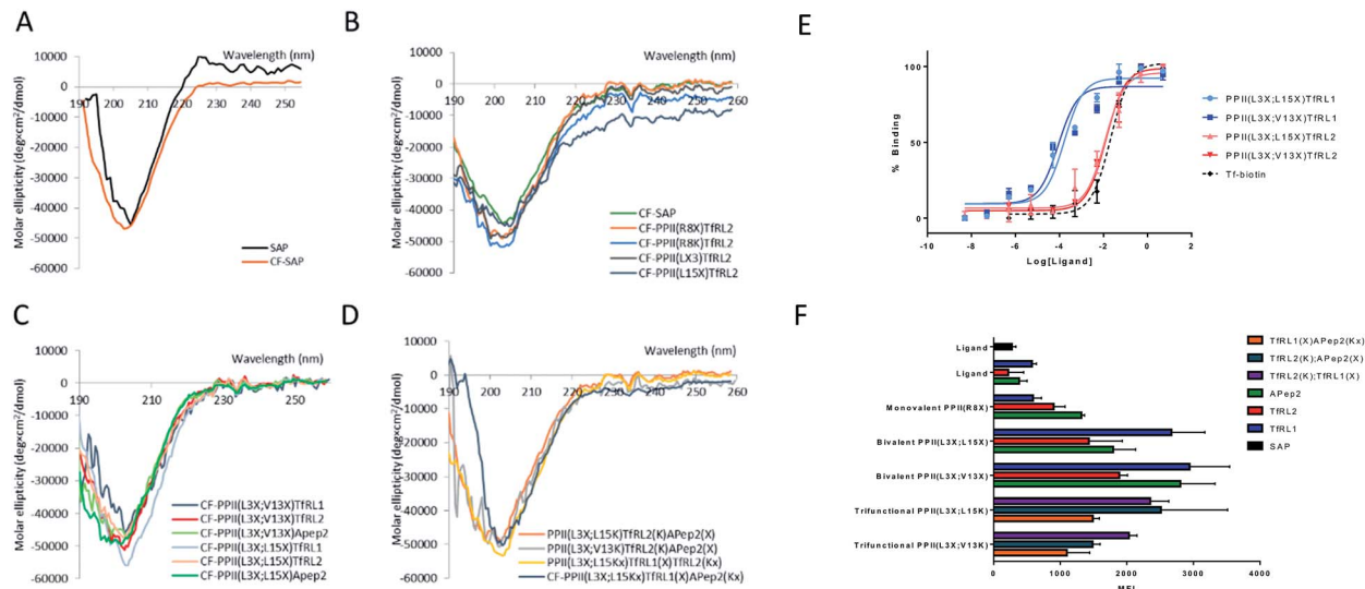
Fig. 2 Properties and uptake capacities of modified SAP vehicle library. (A–D) CD spectra of a selection of FAM labeled delivery vehicles (50 \mu M) in phosphate buffer at pH 7. (A) Wild-type SAP (black) and N-terminally conjugated FAM SAP (CF-SAP; orange). (B) CF-SAP with monovalent vehicles, conjugated to TfRL2 in various positions on the SAP backbone or attached by different conjugation techniques. (C) Bivalent vehicles with ligands incorporated on the same or opposite face of SAP. (D) Trivalent vehicles, incorporating alternative AMT ligands on SAP backbone. (E) ELISA displays the apparent binding affinity ( EC_{50} ) to TfR for Tf (black) or bivalent TfRL1 (blue) and TfRL2 (red) vehicles where ligands are either appended to the same (light) or opposite face (dark). (F) Uptake capacity of FAM labelled vehicles in bEnd.3 cells by flow cytometry. Extracellular fluorescence was quenched by addition of trypan blue. MFI = mean fluorescent intensity.
