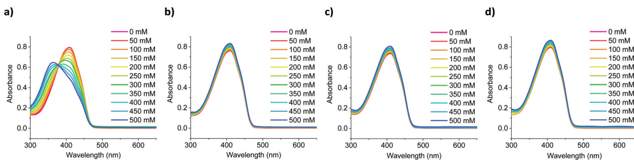
Fig. 3 Representative UV-Vis absorption spectra of S4 in a 1 : 3 mixture of water : tetrahydrofuran ( S4 concentration 4 \times 10^{-5} M) upon incrementing (a) Na + , (b) Li + , (c) K + and (d) Ca 2+ concentrations (0–500 mM).
