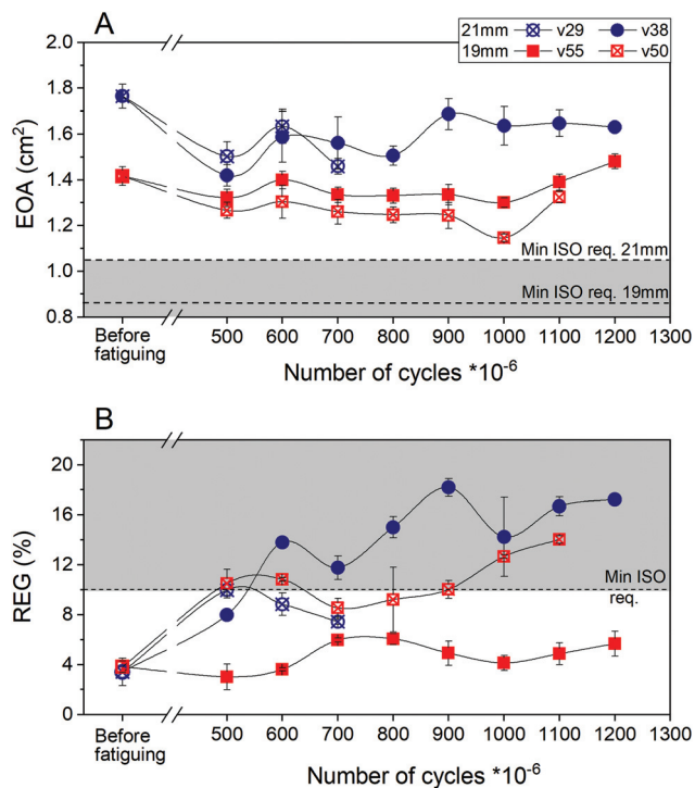
Fig. 4 Hydrodynamic performance of fatigued J6 valves. (A) Effective Orifice Area (EOA); (B) fractional regurgitation (REG). Error bars indicate variation between repeated measurements of the same valve.
