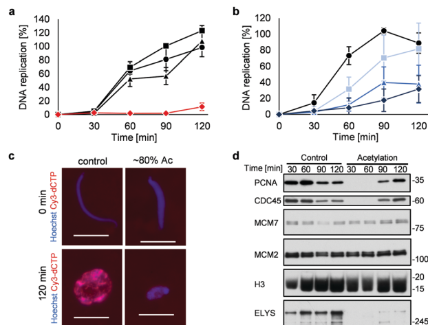
Fig. 4 Synthetic histone acetylation inhibits DNA replication. (a and b) XSC (20 000 sperm per μL) was treated with 2 (30 μM) and 6 (30 mM) for (a) 7 h or (b) the indicated time at 25 °C. After the reaction, control or acetylated XSC was incubated with interphase egg extracts containing radiolabeled [ \alpha - 32 P]-dCTP. The DNA replication kinetics in egg extracts was assessed by the incorporation of radioactivity, determined using a scintillation counter. Data shown are the average and SD (bars) from (a) three or (b) five independent experiments. (a) ●: control; ■: 2 only; ▲: 6 only; ◆: 2 + 6 . (b) ●: control. Reaction time = ■: 0.5 h; ▲: 1 h; ◆: 3 h. (c) and (d) XSC (20 000 sperm per μL) was treated with 2 (30 μM) and 6 (30 mM) for 7 h. (c) Control or acetylated XSC was incubated with interphase egg extracts containing Cy3-dCTP. After incubation, the samples were fixed and DNA was visualized with Hoechst 33258 (blue image). DNA replication was monitored as the incorporation of Cy3-dCTP (red image) into DNA. The scale bar represents 20 μm. (d) Control or acetylated XSC was incubated with interphase egg extracts. Chromatin was isolated from the egg extracts at the indicated times and the chromatin samples were analyzed by immunoblotting using the indicated antibodies.
