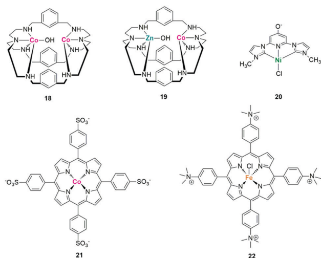
Fig. 15 Representative structures of several \text{CO}_2 photoreduction complex catalysts.
