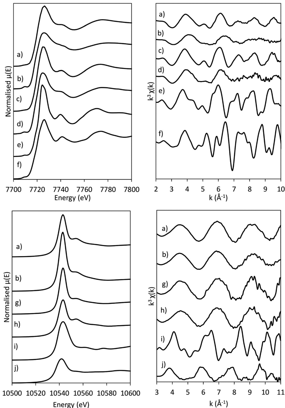
Fig. 4 XANES spectra (left) and k^3 -weighted chi-curves (right) of the (a) as-synthesised CoRe-gel, (b) annealed CoRe-gel, (c) as-synthesised Co-gel, (d) annealed Co-gel, (e) Co(OH) 2 , (f) CoO, (g) annealed Re-gel, (h) NH 4 ReO 4 , (i) ReO 3 and (j) ReO 2 at the Co K-edge (top) and at the Re L III -edge (bottom).
