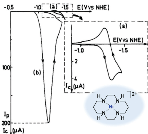
Fig. 13 Cyclic voltammograms of [\text{Ni}(\text{cyclam})]^{2+} ( 40 , 1 mM) in 0.1 M \text{KClO}_4 (pH 4.5) under \text{N}_2 (curve a) or \text{CO}_2 (curve b) on a hanging Hg electrode. Scan rate: 0.1 \text{ V s}^{-1} . Reprinted with permission from ref. 210. Copyright 1986 American Chemical Society.
