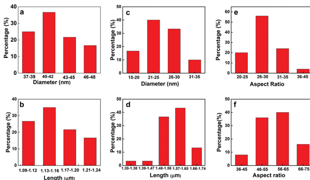
Fig. 2 Diameter, length and aspect ratio distribution of Te NWs at 120 °C for 21 h. (a), (b) and (e) 0.1 gm PVP and 0.75 mL ascorbic acid (c), (d) and (f) 0.2 gm PVP and 1.5 mL ascorbic acid.
