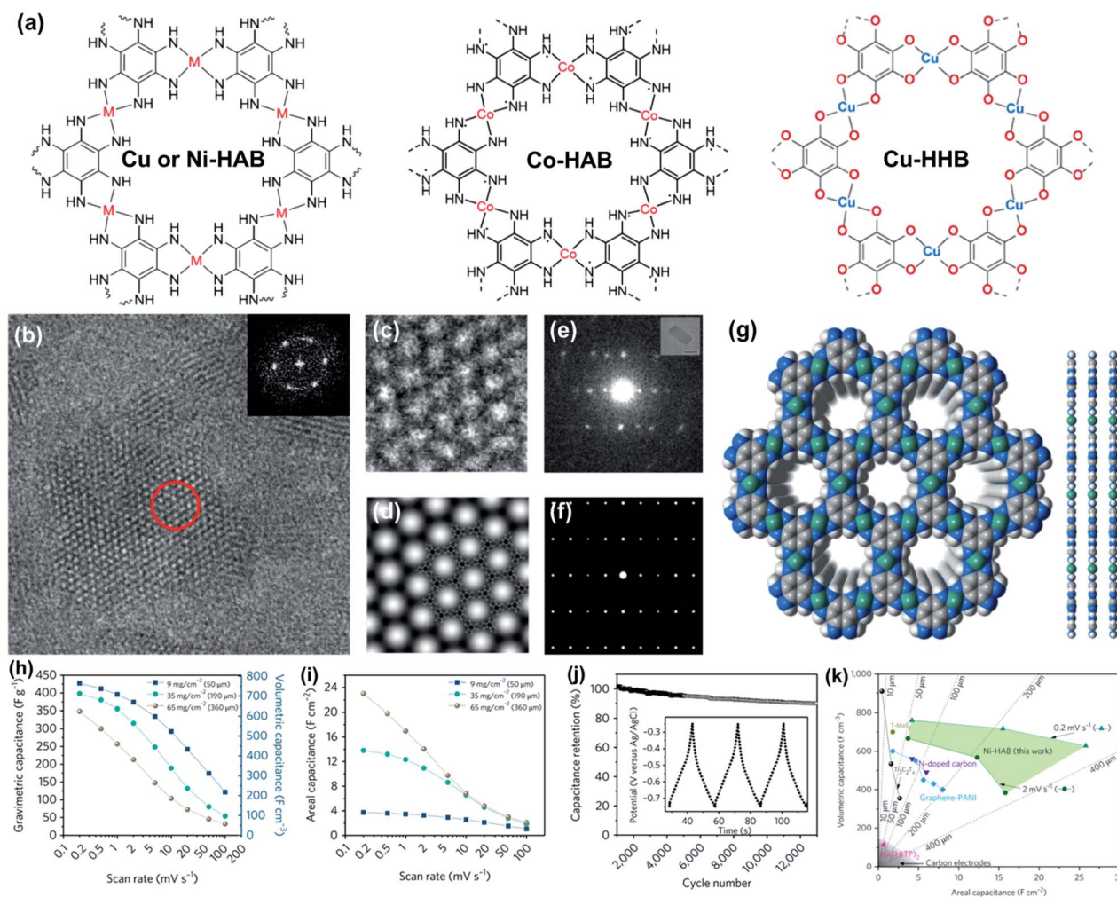
Fig. 15 (a) 2D MOFs in M_3(C_6H_6)_2 ( M = \text{Cu, Co, and Ni} . X = \text{NH, S, and O} ) family. (b) HR-TEM image of Cu-HAB along [001] that shows a hexagonal pore packing with d_{100} = 1.15 \text{ nm} ( a = 1.33 \text{ nm} ). Scale bar, 10 nm. Inset: Fourier transform of the image. (c) HR-TEM image of the region within the red circle in (b). (d) Symmetry-imposed and lattice-averaged image calculated from the HR-TEM image. Embedded is the eclipsed structure model of Cu-HAB. Scale bar, 2 nm. Experimental (e) and simulated (f) electron-diffraction pattern (eclipsed model) of Cu-HAB viewed along [-110] . Scale bar 5 \text{ nm}^{-1} . Inset (e): the crystal from which the electron-diffraction pattern was taken. Scale bar, 50 nm. (g) A space-filling model of the Cu-HAB model. Blue, grey, green and white spheres represent N, C, Ni and H atoms, respectively; a.u.: arbitrary units. (h) Gravimetric and volumetric rate performance for Ni-HAB pellet electrodes with different areal densities of 9, 35, and 65 \text{ mg cm}^{-2} . (i) Areal rate performance for the Ni-HAB electrodes with different weight loadings. (j) Capacitance retention data collected by galvanostatic charge–discharge at 10 \text{ A g}^{-1} . Inset: galvanostatic charge–discharge profiles. (k) Comparison of the volumetric and areal capacitances of Ni-HAB additive-free electrodes (green area) with the performance of other materials. Reproduced with permission. 119 Copyright©2018 Nature Publishing Group.
