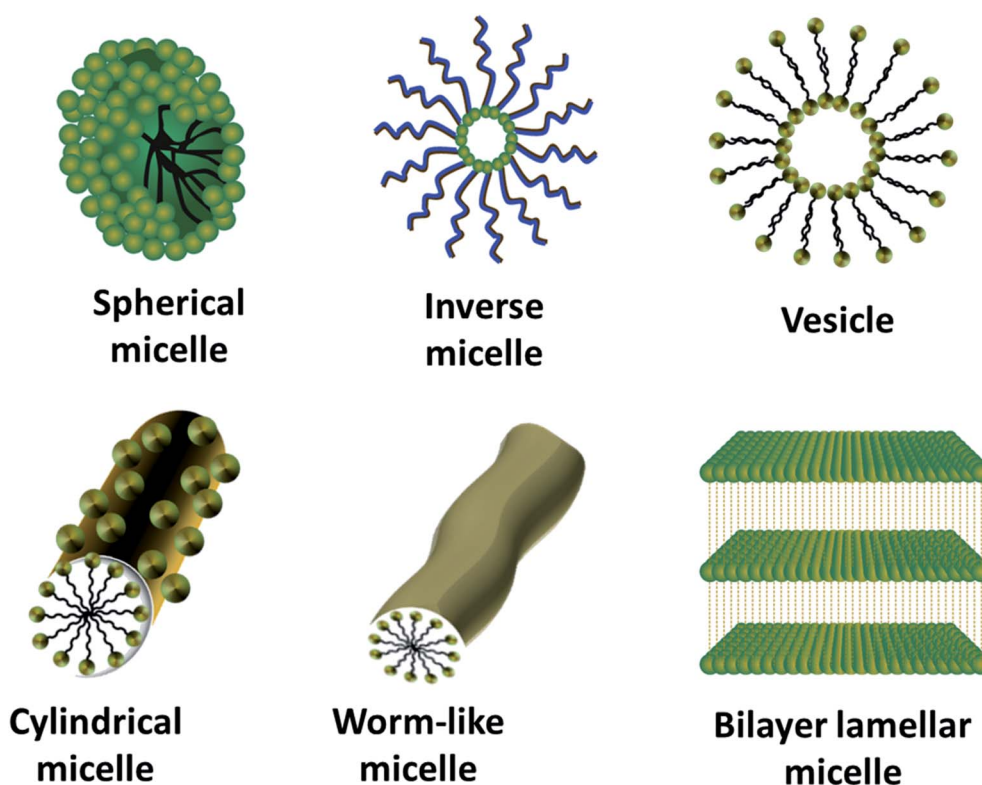
Fig. 4 Schematic representation of different-shaped micelles ranging from spherical micelles ( g \leq 1/3 ) to bilayer lamellar micelles ( g = 1 ).
