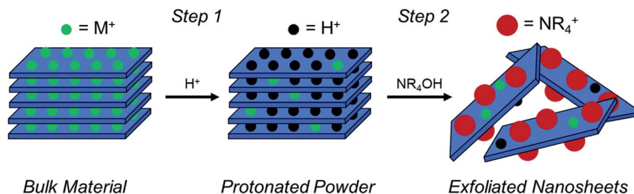
Fig. 1 A schematic of the two-step soft-chemical exfoliation process to obtain atomically thin TMO nanosheets from bulk TMOs in which nanosheets are held together by coulombic interactions. Step one uses a protic acid ( \text{H}^+ ) to replace alkali ions with protons in the interstices of the layered structure, producing a “protonated powder”. The second step uses a hydroxide bearing a bulky cation [ i.e. , a quaternary amine ( \text{NR}_4\text{OH} )] to promote osmotic swelling and exfoliation of individual TMO nanosheets.
