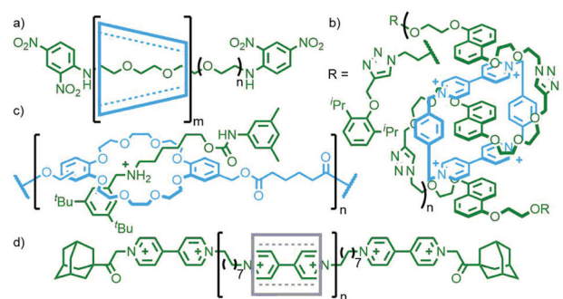
Fig. 37 Main chain poly[n]rotaxanes prepared via the capping approach: (a) Harada's seminal PEG/ \alpha -CD polyrotaxane; (b) Stoddart's donor-acceptor system; (c) an alternative design in which the macrocycle is incorporated in the polymer backbone by Takata; (d) Ogoshi's pillarane polyrotaxane with viologen-based axle.
