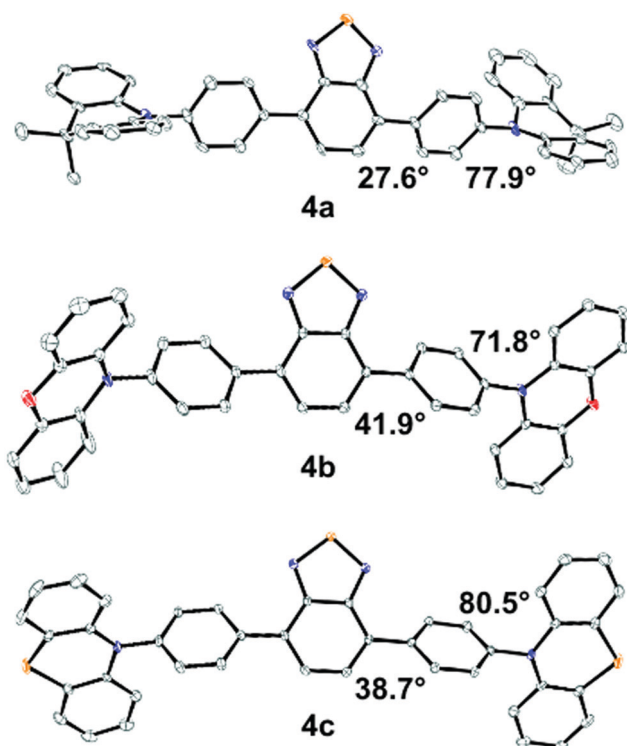
Fig. 2 Molecular structures of 4a–c with thermal ellipsoids at the 50% probability level. Hydrogen atoms have been omitted for clarity. Carbon = grey, nitrogen = blue, oxygen = red, sulfur = yellow. Respective average BTD-phenyl and phenyl-donor dihedral angles are shown.
