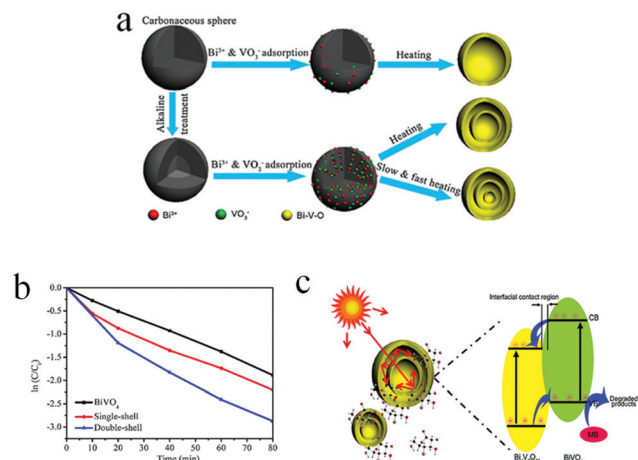
Fig. 44 (a) Schematic illustration of the synthesis procedure of multi-shelled Bi-V-O hollow microspheres. (b) Catalytic performance of solid BiVO 4 and single- and double-shelled Bi-V-O hollow microspheres. (c) Schematic diagram of the photocatalytic mechanism of the hetero-structures of multishelled Bi-V-O hollow microspheres. Reprinted from ref. 234 with kind permission.
