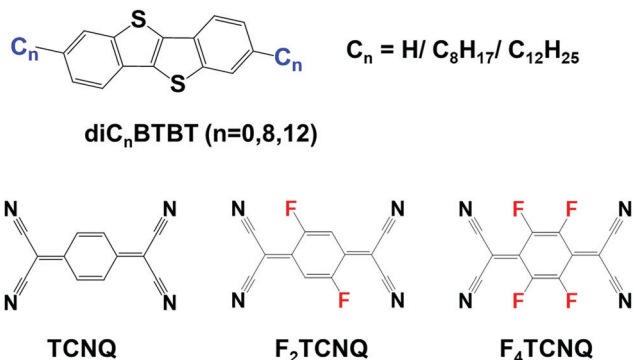
Fig. 1 Chemical structures of the BTBT ( n = 0 , \text{C}_n \equiv \text{H} ), \text{diC}_8\text{BTBT} ( \text{C}_8 \equiv \text{C}_8\text{H}_{17} ), and \text{diC}_{12}\text{BTBT} ( \text{C}_{12} \equiv \text{C}_{12}\text{H}_{25} ) donors as well as the TCNQ, \text{F}_2\text{TCNQ} , and \text{F}_4\text{TCNQ} acceptor molecules.
