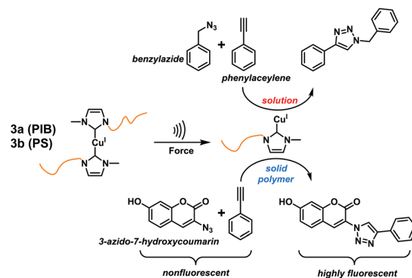
Fig. 3 Mechanochemical activation of latent copper(I)-NHC catalysts ( 3a , 3b ) both in solution and in the solid polymer matrix; the activated catalysts then catalyze "click" reactions. Reproduced with permission. 40 Copyright 2015, John Wiley and Son.
