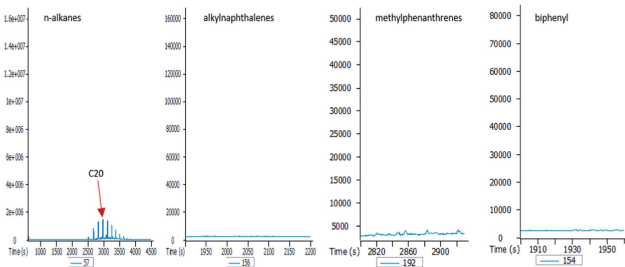
Fig. 8 Partial mass chromatograms ( m/z 57, 156, 192 and 154) of the E2 leachates, showing limited ( n -alkanes) or no elution of diesel fuel hydrocarbons ( C_2 alkylnaphthalenes, methylphenanthrenes, biphenyl). E20: diesel fuel containing 20% ethanol (v/v).
