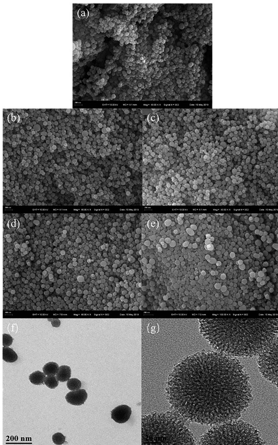
Fig. 2 SEM images of HBPS- \text{NH}_2 (a), HBPS-Ph (b), HBPS-COOH (c), HBPS- \text{C}_6\text{H}_{13} (d) and HBPS- \beta -CD (e) and TEM images of HBPS (f and g).
