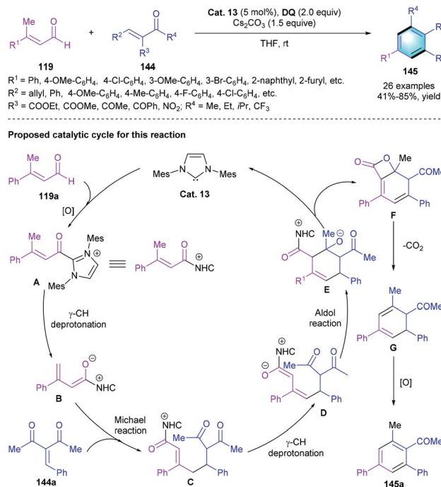
Scheme 42 NHC-catalyzed [3 + 3] benzannulation to synthesize polyfunctionalized benzenes.
