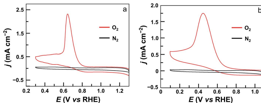
Fig. 4 CVs of GC electrodes loaded with 5 \mu L ink of 1 (a) and 2 (b) under N 2 (black) and O 2 (red) in 0.5 M H 2 SO 4 solution. Conditions: GC working electrode, 50 mV s -1 scan rate, 20 °C.
