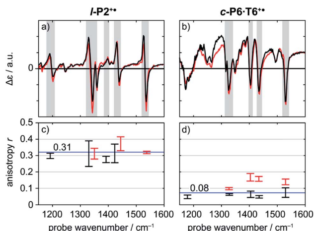
Fig. 5 Normalized TRIR spectra of \text{I-P2}^{++} (a) and \text{c-P6}\cdot\text{T6}^{++} (b) with pump centered on C \equiv C stretch mode ( 2100 \text{ cm}^{-1} ) (black) and on P 1 polaron band ( 3250 \text{ cm}^{-1} for \text{I-P2}^{++} , 2500 \text{ cm}^{-1} for \text{c-P6}\cdot\text{T6}^{++} ) (red) with probe delay 0.8 \text{ ps} . Anisotropy values of the selected TRIR regions (grey area in the spectra) of \text{I-P2}^{++} (c) and \text{c-P6}\cdot\text{T6}^{++} (d) are plotted for both pump positions, with error bars indicating standard error.
