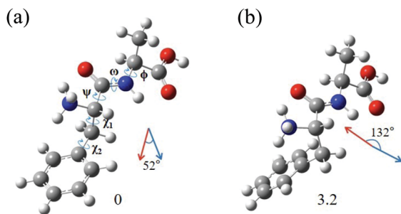
Fig. 7 Structures of conformers (a) I and (b) II of L-H + PheAla optimized at the CAM-B3LYP/6-311+G(d,p) level. The dihedral angles of the structures are labeled as \psi , \omega , \phi , \chi_1 , and \chi_2 . The red and blue arrows represent \mu and m , respectively. The numbers at the bottom are the relative energies of the conformers in kJ mol -1 .
