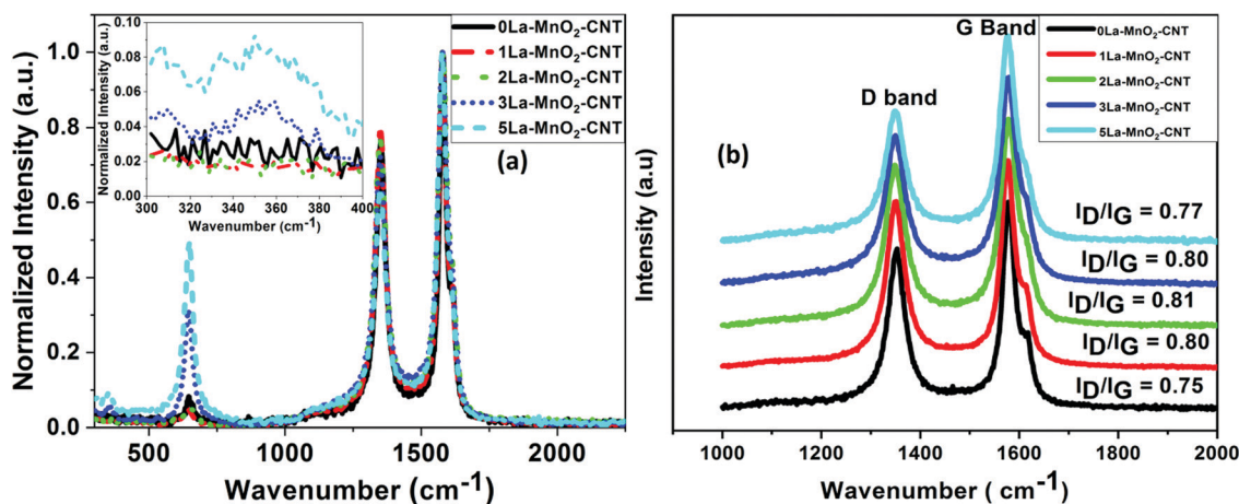
Fig. 2 Raman spectra of undoped and La-doped MnO 2 -CNT (a); Raman spectra showing the D band and G band of undoped and La-doped MnO 2 -CNT (b).
