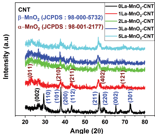
Fig. 1 XRD pattern of undoped and La 3+ :MnO 2 -CNT nanohybrid.
