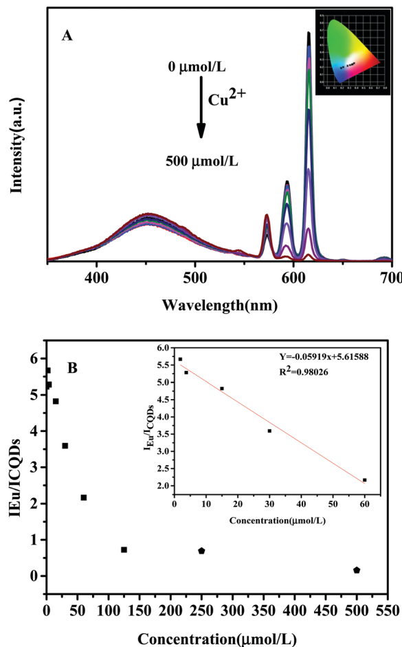
Fig. 6 The emission spectra of the Eu-DPA-CQDs immersed in aqueous solutions of Cu 2+ ions at different concentrations ( \lambda_{ex} = 285 nm).
