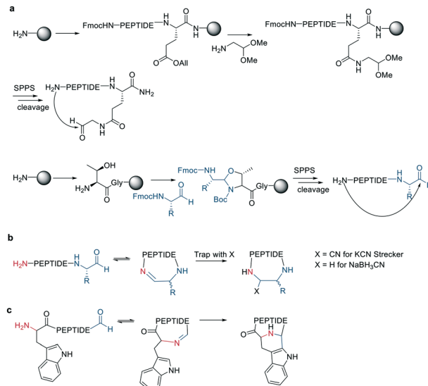
Scheme 9 Peptide cyclization via imine formation and subsequently trapping of the imine. a : On-resin strategies to generate the aldehyde. b : General reaction scheme of imine formation and trapping. c : Trapping via Pictet-Spengler.
