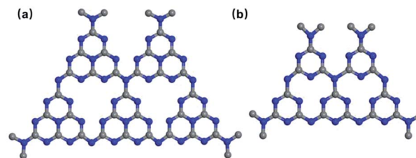
Fig. 1 (a) Tri- s -triazine and (b) s -triazine structure of g-C 3 N 4 .
