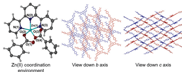
Fig. 3 Left: The zinc(II) coordination environment in 3 showing only the terpy region of the coordinating Hc bt ligand and coordinating benzoate groups of neighbouring Hc bt ligands. Ellipsoids are shown with 50% probability. Right: Two stacked 2D sheets (shown in red and blue) of [Zn(Hc bt )] in 3 as viewed down the crystallographic b and c axes. Solvent molecules present within the structure have been removed for clarity.
