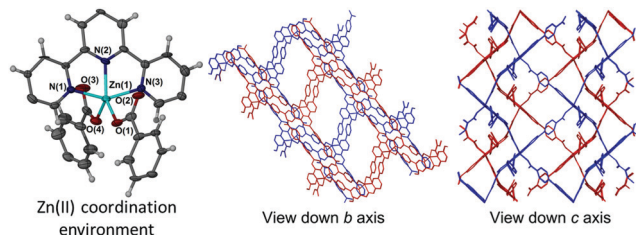
Fig. 2 Left: The zinc(II) coordination environment in 2 showing only the terpy region of the coordinating Hc bt ligand and coordinating benzoate groups of neighbouring Hc bt ligands. Ellipsoids are shown with 50% probability. Right: Stacked 2D sheets (shown in red and blue) of [Zn(Hc bt )] in 2 as viewed down both the crystallographic b and c axes. Lattice solvents present within the channels have been removed for clarity.
