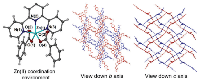
Fig. 1 Left: The zinc(II) coordination environment of 1 showing only the terpy region of the coordinating Hc bt ligand and coordinating benzoate groups of neighbouring Hc bt ligands. Ellipsoids are shown with 50% probability. Right and centre: Two stacked 2D sheets (shown in red and blue) of [Zn(Hc bt )] in 1 as viewed down the crystallographic b and c axes. Lattice solvents present within the channels have been removed for clarity.
