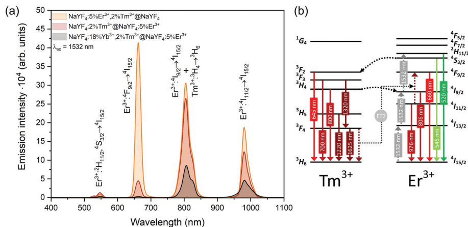
Fig. 7 (a) Emission of synthesised core@shell NPs under 1532 nm laser excitation ( 15 \text{ W cm}^{-2} ). (b) Possible energy transfers in NPs doped with \text{Er}^{3+} and \text{Tm}^{3+} ions under 1532 nm laser excitation.
