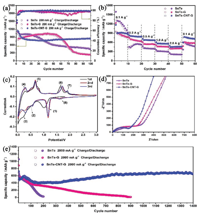
Fig. 4 (a) Cycling performance and coulombic efficiency of the three samples at 200 \text{ mA g}^{-1} . (b) Rate performance of all samples. (c) CV curves of the SnTe-CNT-G anodes at 0.2 \text{ mV s}^{-1} . (d) Nyquist plots of all electrodes before cycling. (e) Cycling performance at 2000 \text{ mA g}^{-1} .
