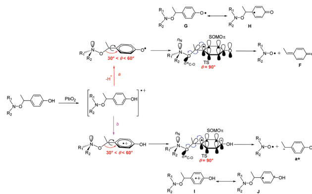
Scheme 6 Generation of nitroxide from alkoxyamine through a PCET process coupled with the \beta -fragmentation of phenoxyl radical (route a) and the mesolysis of radical cation (route b), and geometrical parameters and orbital interaction at their respective TS.
