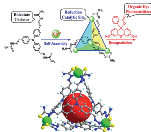
Fig. 24 Supramolecular cages self-assemble when a ligand and Co 2+ ions are combined in a 1 : 1 stoichiometry. The cage encapsulates an organic fluorescein photosensitizer in a following step. The assembly is an efficient light drive proton reduction catalyst. Used with permission from ref. 112.
