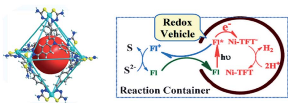
Fig. 20 The supramolecular Ni-TFT cage (left) has ample space to encapsulate fluorescein (red ball). A scheme of the overall \text{H}_2\text{S} splitting at pH 11–13 is depicted (right). The cage encapsulates fluorescein (FL) and expels the dye as it is oxidized. Used with permission from ref. 102.
