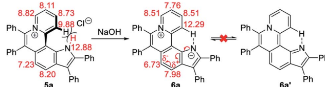
Scheme 3 Conformation transformation from 5a to 6a and chemical shifts of their characteristic protons.
