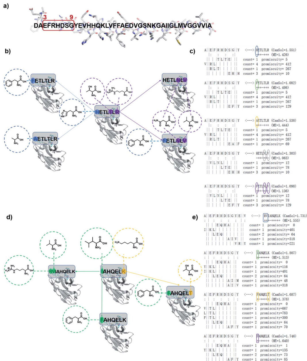
Fig. 1 Schematic representation of designed antibodies (DesAbs) against Aβ 42 aggregation. (a) Target epitope within the Aβ 42 peptide sequence (residues 3–9). (b) A first group of DesAbs with different CDR3 regions is based on the -ETL-L- motif and, a second group (d) on the -AHQEL- motif. These two groups differ also in the predicted backbone–backbone hydrogen bonding pattern they form with the target epitope (colon symbols in (c) and (e)). In the group based on the -ETL-L- motif, we mutated systematically three positions, two at the N-terminus (blue) and one at the C-terminus (purple) to obtain the five DesAbs shown in panel (b), which include the parent DesAb-HETLTLR. 16 (c and d) In the group based on the -AHQEL- motif, we mutated two positions, one at the N-terminus (green) and one at the C-terminus (yellow) to obtain the four DesAbs shown in panel (d). (c and e) Fragment-composition of the designed peptides grafted in the CDR3 of the DesAbs, as resulting from the cascade procedure, together with their count and promiscuity scores (for details see ref. 18). The sequence of the target epitope (residues 3–9 of Aβ 42 ) is shown to the left; colon marks denote residues predicted to be involved in hydrogen-bonds with the designed peptide, whose sequence is shown to the right, while the fragments composing it are below the target epitope; as the binding is antiparallel, these fragments are represented in the C- to N-terminus direction. 18 The selected mutations are circled, and result from the choice of different fragments in the cascade procedure. Complementary peptide candidates with low predicted solubility (CamSol score) were not considered.
