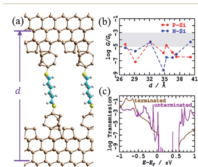
Fig. 4 Modelling the STMBJ experiment, using regular unterminated silicon tips on each unterminated electrode. (a) 2D ( 3 \times 3 ) model for tips spanned by S(CH_2)_6S at d = 37.37 \text{ \AA} ; Si-brown, S-yellow, C-cyan, H-white. (b) Conductivity at zero voltage for P-type and N-type silicon at 0 K; the shaded region shows the observed conductance found throughout extensions of 3–10 \text{\AA} for P-type Si. See ESI† Fig. S4 for more information. (c) Comparison of the transmission for P-type Si, as a function of electron energy from the Fermi energy, at d = 32.17 \text{ \AA} , from this unterminated series to that for the analogous terminated structure (Fig. 3, ESI† Fig. S3).
