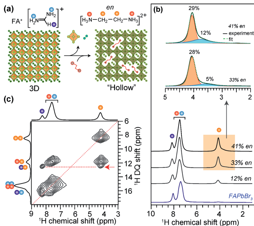
Fig. 8 Large cation incorporation in hollow \text{FAPbBr}_3 : (a) schematic of the formation of hollow perovskites, (b) solid-state ^1\text{H} MAS NMR spectra of \text{FAPbBr}_3 and ( en ) \text{FAPbBr}_3 ( en content = 12%, 33% and 41% of available sites) hollow perovskites together with the assignment of signals corresponding to \text{FA}^+ and en protons depicted in color dots as shown in the figure inset. (c) 2D ^1\text{H} - ^1\text{H} DQ-SQ correlation NMR spectra of 41% en / \text{FAPbBr}_3 exhibit the cross peaks (red arrow) indicating the sub-nm molecular proximity between \text{FA}^+ and en . Adapted with permission from ref. 373. Copyright 2021 American Chemical Society.
