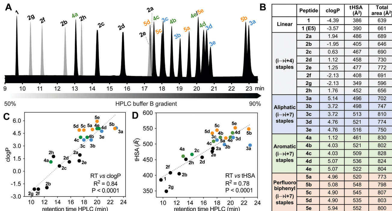
Fig. 6 Hydrophobicity of 1 , 2a–h , 3a–e , 4a–e , 5a–e . A. HPLC analysis showing retention time for each peptide using a C18 column (Phenomenex Luna), at 1 \text{ mL min}^{-1} flow and 2.5 buffer B (0.1% TFA, 90% ACN) gradient per minute. B. Calculated parameters: logP (clogP), total hydrophobic surface area (tHSA) and total surface area for each peptide. C and D. Correlation between clogP (2D hydrophobicity) and HSA (3D hydrophobic surface area) calculated for each peptide vs. experimental HPLC retention.
