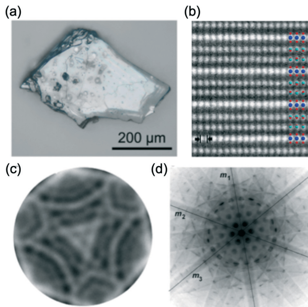
Fig. 4 (a) Optical micrograph image of a single crystal of \text{InGaO}_3(\text{ZnO})_{1.1} . (b) HAADF image of \text{InGaZnO}_4 in [1\bar{1}00] orientation with structure model. The blue, red, and light green circles represent In, Zn/Ga, and O atoms, respectively. Cation columns of In (bright) and Zn/Ga (medium bright) are well resolved indicating the cation layer stacking in \text{InGaZnO}_4 . A spacing of 0.16495 nm of the (2\bar{1}\bar{1}0) prism planes is shown. (c) Central CBED disc and (d) whole pattern results suggest 3m symmetry. Panels (a-d) are reprinted with permission from ref. 46. © 2014 Elsevier.
