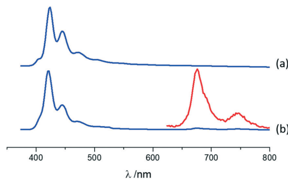
Fig. 5 Normalized luminescence spectra in the solid state for (a) pure A and (b) A \cdot (I2F4)_2 (arbitrary units on the y -axis). \lambda_{\text{exc}} = 380 \text{ nm} . The phosphorescence spectrum in the 650–800 nm region, isolated with a gated detection, is magnified in the inset for A \cdot (I2F4)_2 . The phosphorescence emission is clearly evident in A \cdot (I2F4)_2 compared to solid anthracene, where no phosphorescence was detected.
