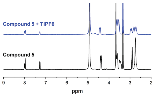
Fig. 3 1 H NMR binding experiment with compound 5 and TlPF 6 in MeOD.
