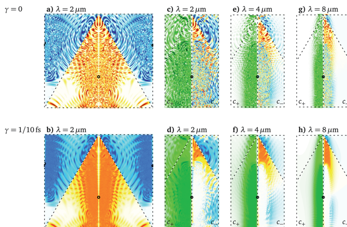
Fig. 5 q -resolved conduction-band populations for selected wavelengths ( \lambda = 2, 4, 8 \mu\text{m} ). Shown is c(q) , for \lambda = 2 \mu\text{m} only, and in compact form, cf. sketch in Fig. 1, the excitation c_+(q) and the polarization c_-(q) . We show both results with (lower row) and without (upper row) damping. Color scales are given in Fig. 1d.
